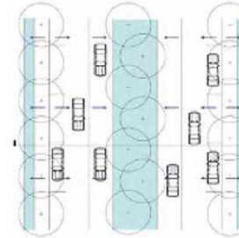
Bioswale with Open Section
