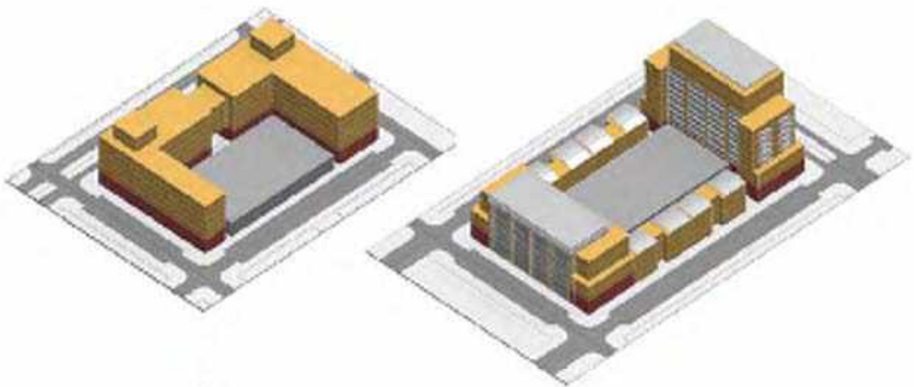
Examples of parking structures internal to blocks and laminated or veneered by buildings
