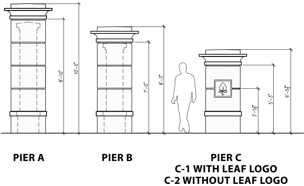
Pier Type Diagram
