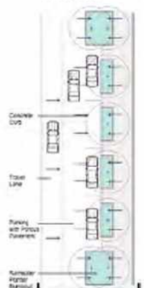
Rainwater Planter with Bumpout
