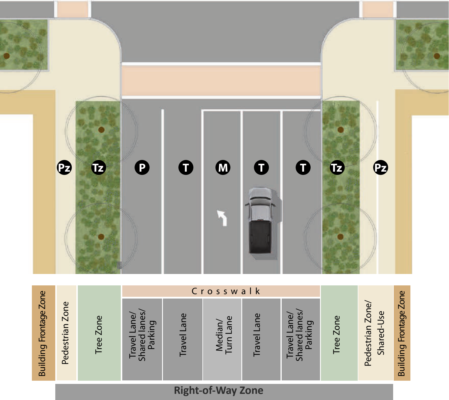
Complete Streets Diagram This diagram is for illustrative purposes only.
