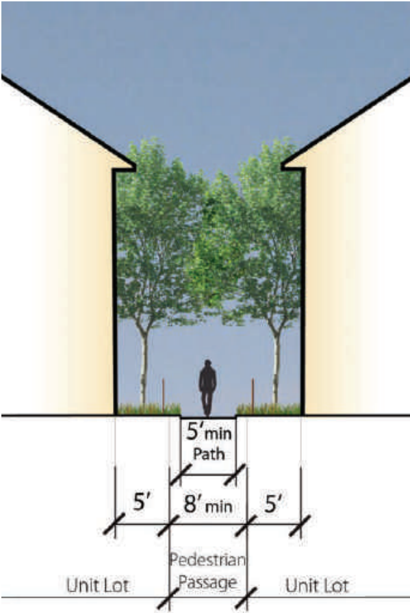
Pedestrian Passage Typical Section
