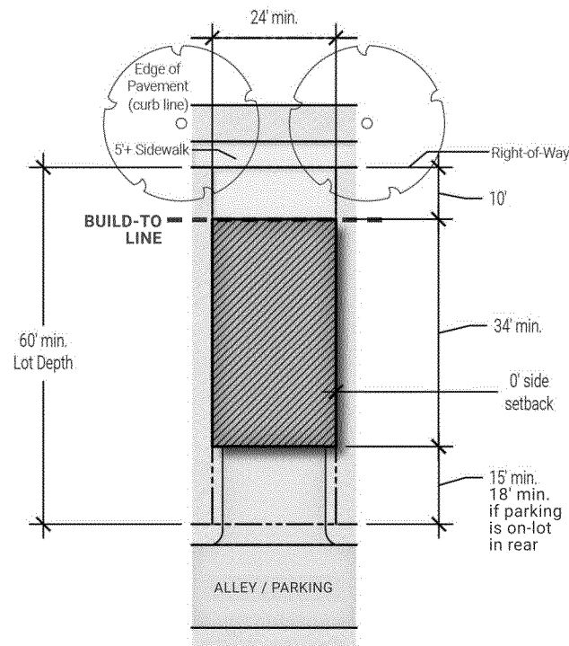
Live-Work Integral Garage - Mid-Block
