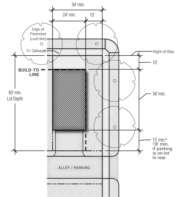
Live-Work Integral Garage - Corner Lot
