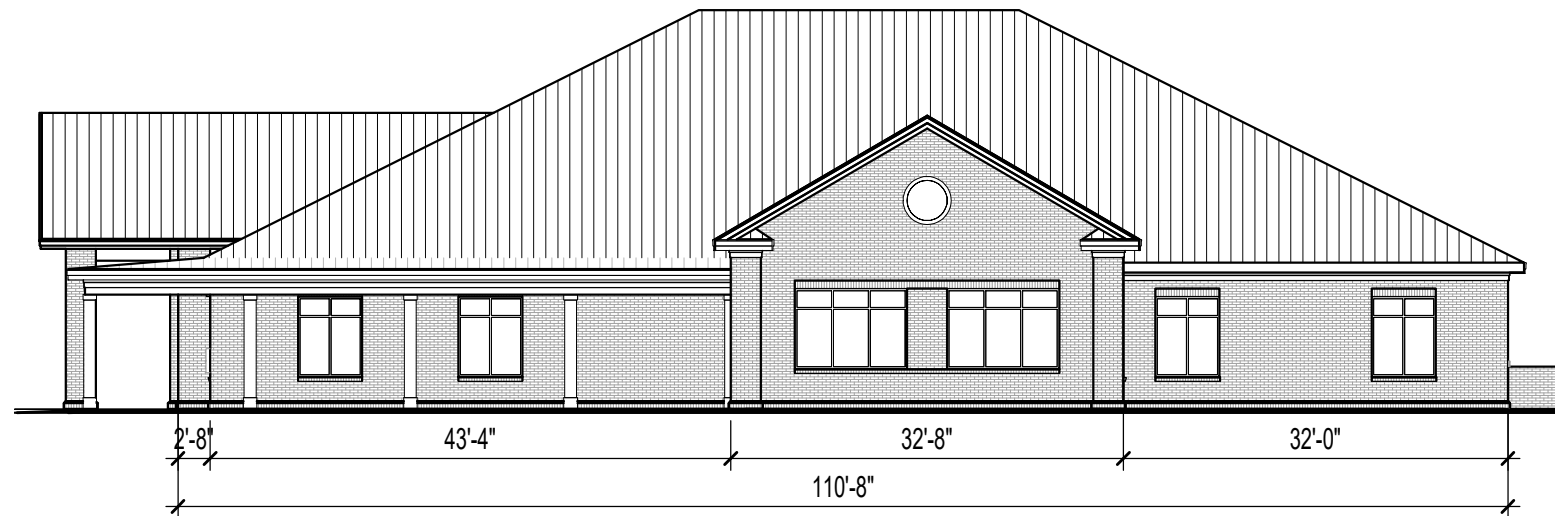
2 RIGHT ELEVATION PR4 1/16" = 1'-0"
