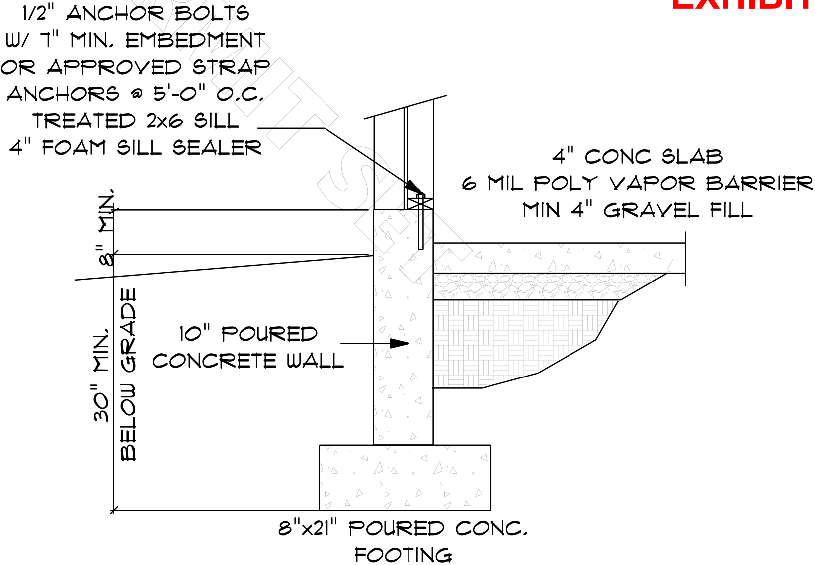
GARAGE WALL SECTION
