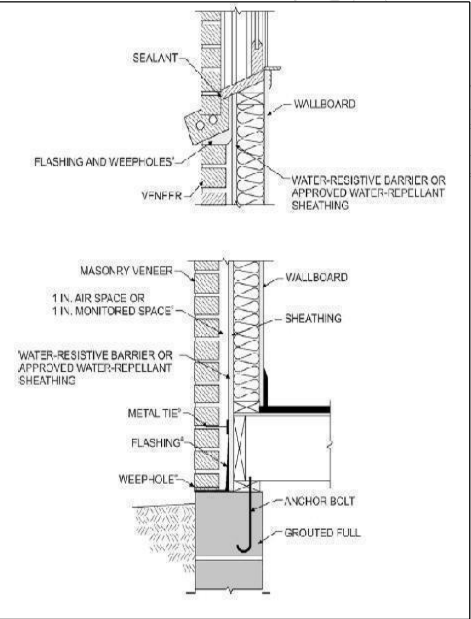
BRICK VENEER DETAIL
