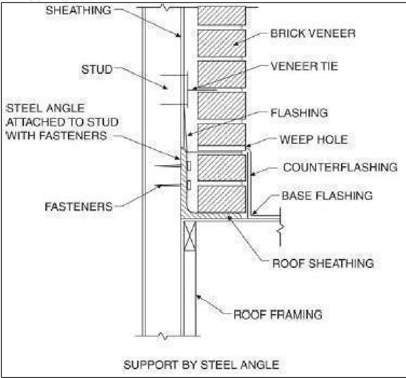
BRICK LINTEL DETAIL
