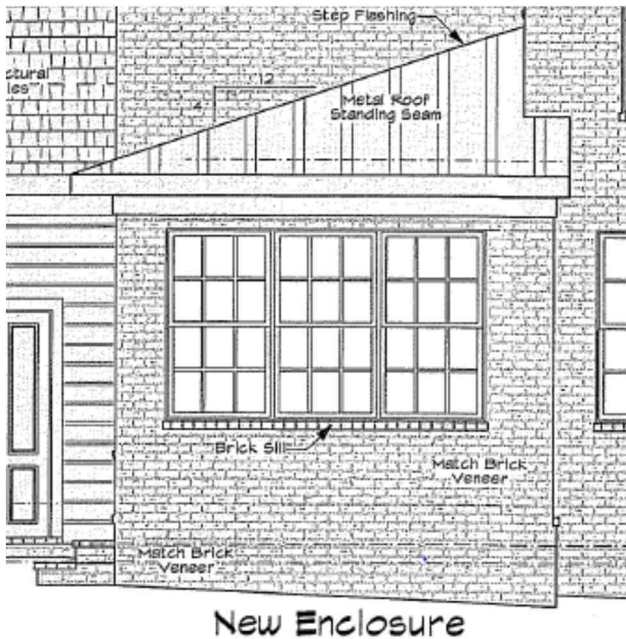
Left Elevation (Side)
