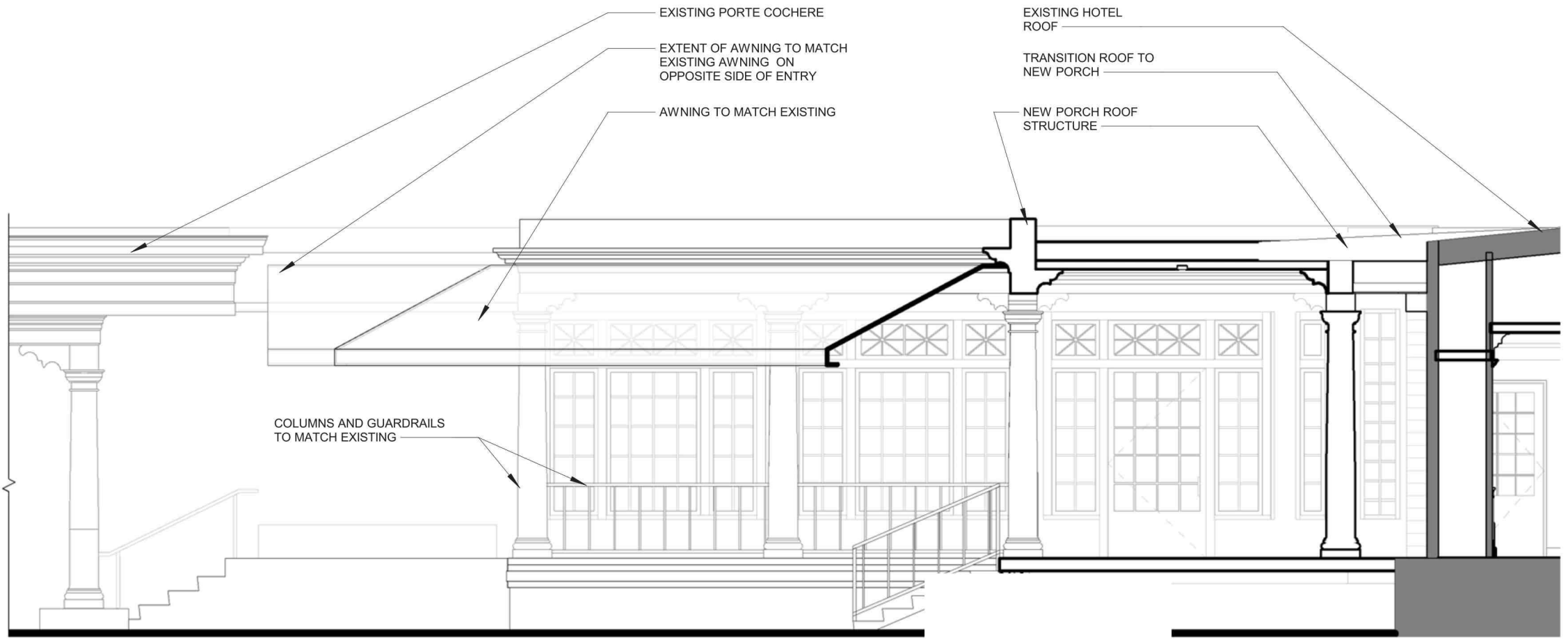
Veranda North Elevation
