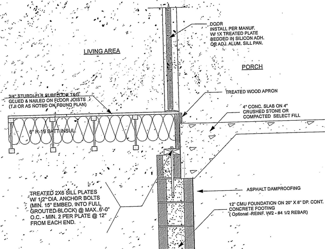
2 TYP. SECTION THRU EXTERIOR WALL @ CONCRETE PORCH Scale: 3/4" = 1'-0"
