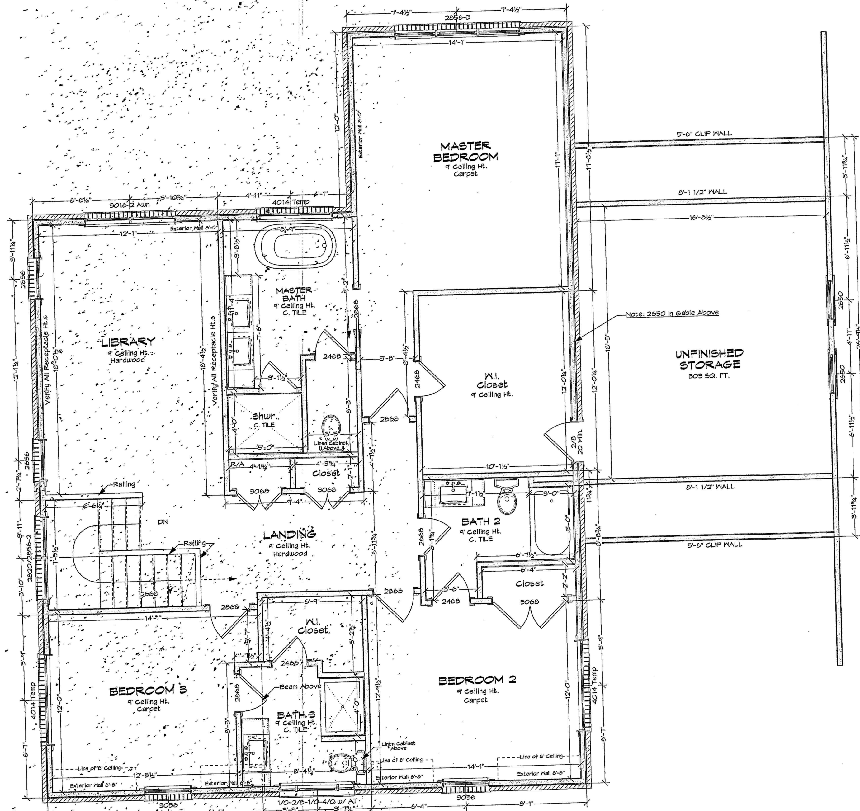
2 Second Floor Plan Scale: 1/4" = 1'-0"
