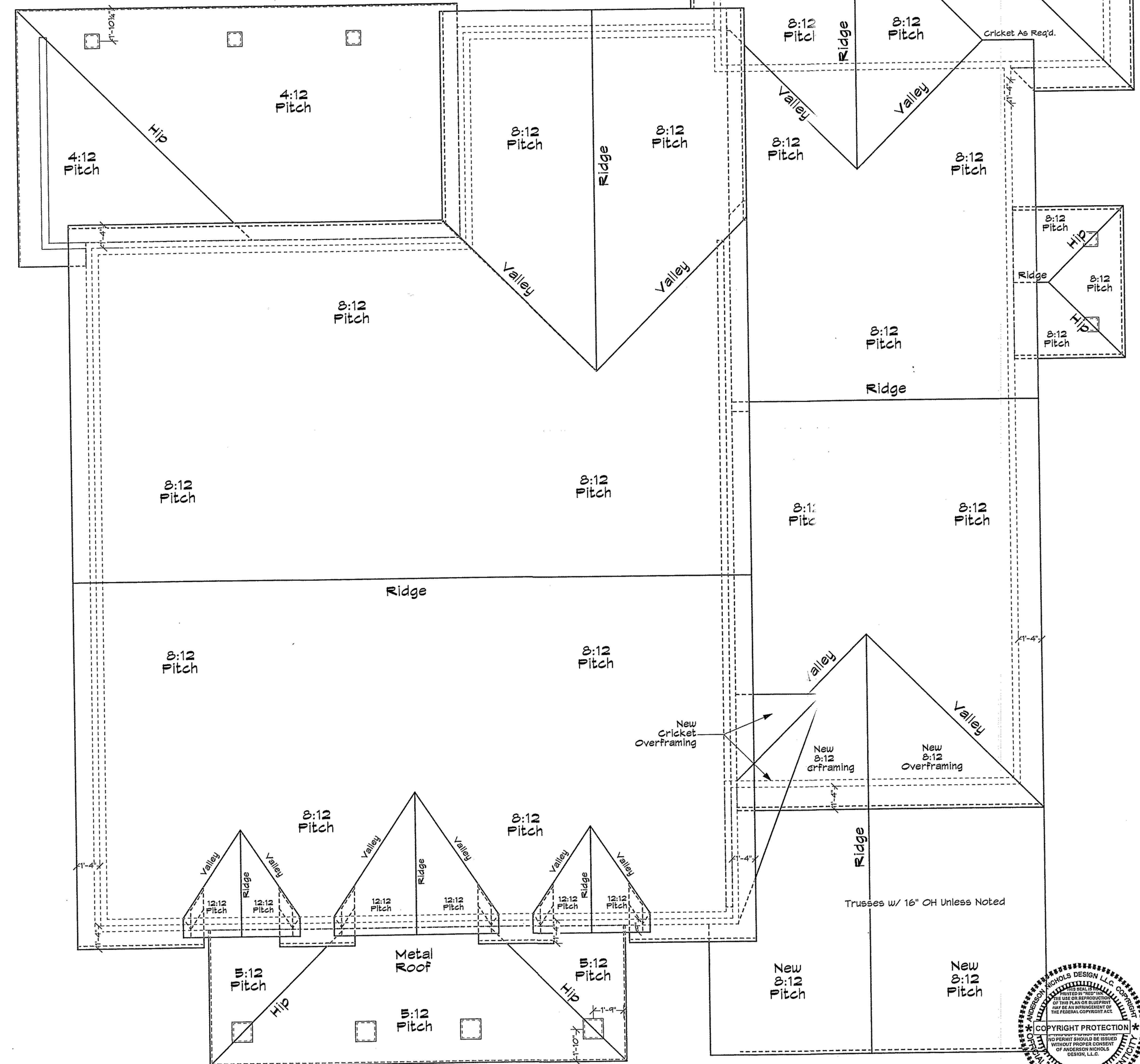
2 New Roof An Addition (Engineered Trusses) Scale: 1/4\" = 0'
