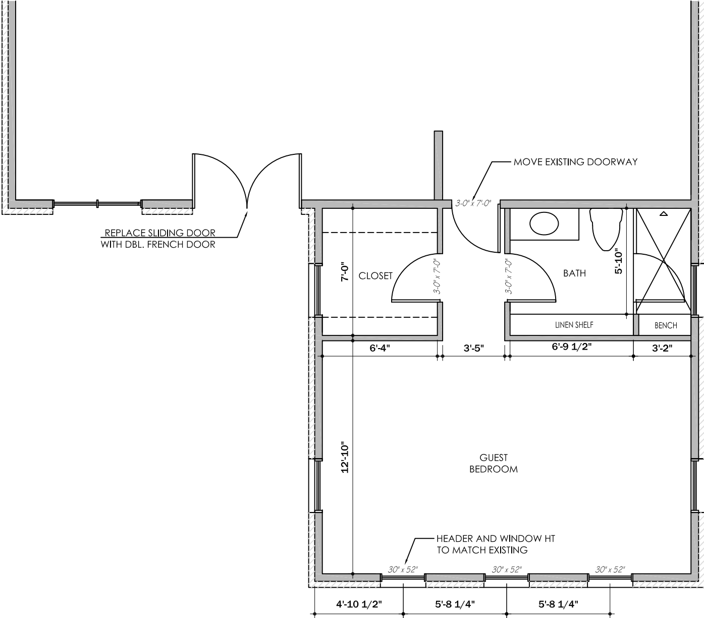
2 PROPOSED CONVERSION SCALE: 3/16" = 1'-0"
