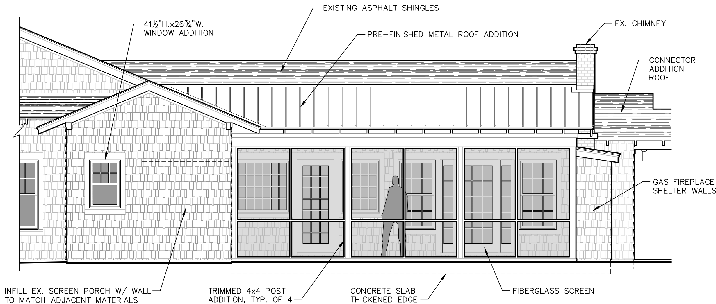
SCREEN PORCH ADDITION EXTERIOR ELEVATIONS SCALE: 1/4" = 1'-0"
