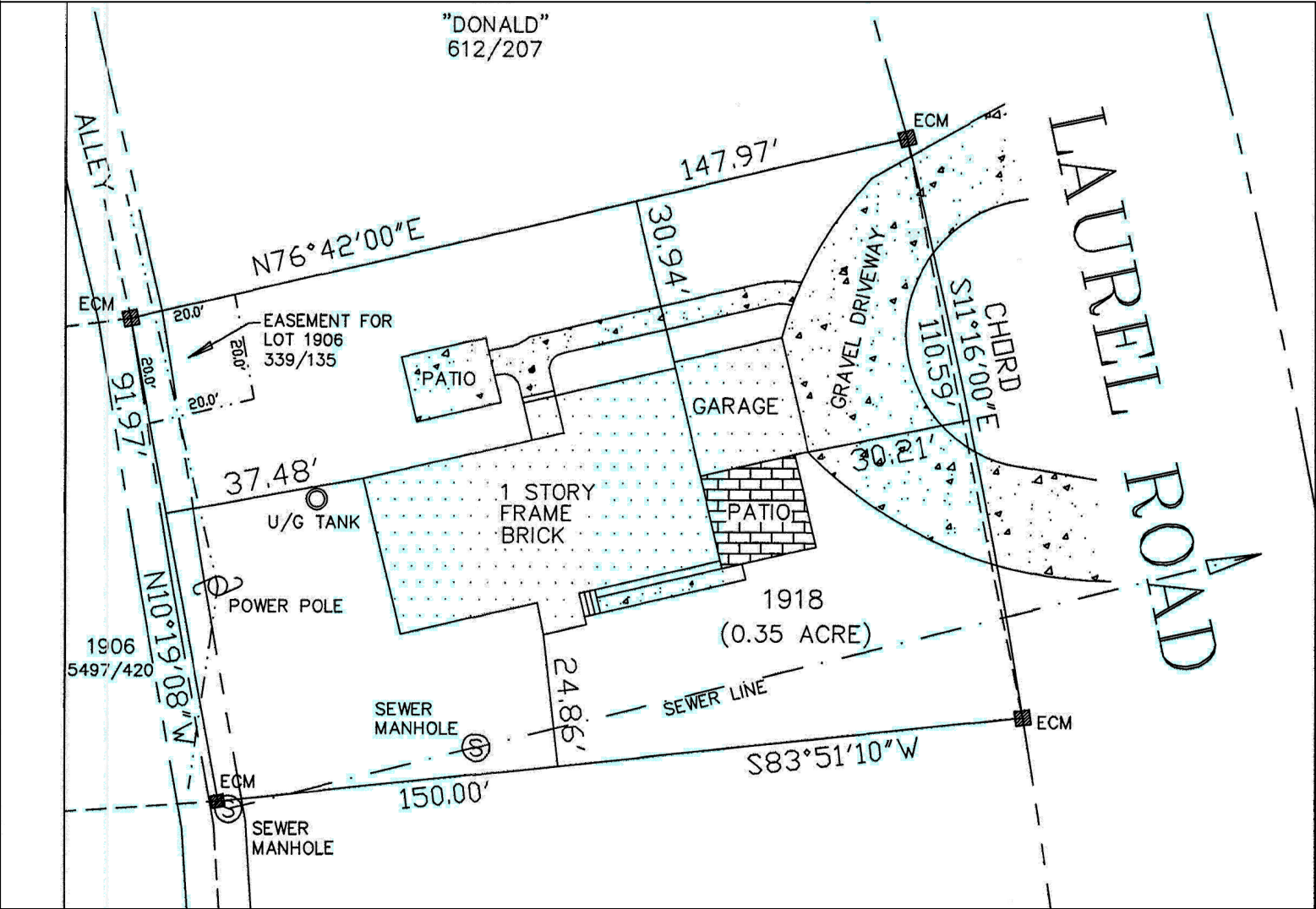
EXISTING SITE PLAN - FOR REFERENCE ONLY SCALE: NTS
