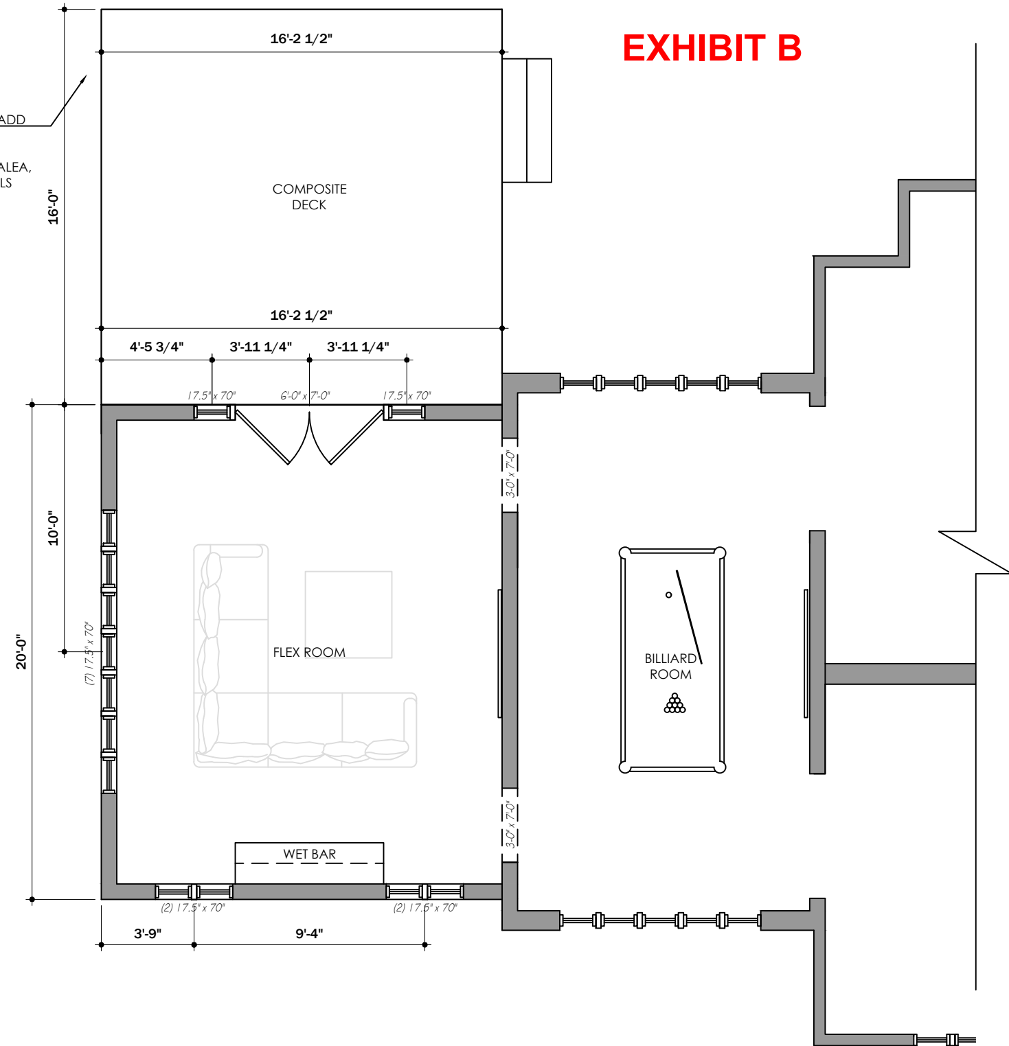
2 PROPOSED ADDITION - FIRST FLOOR SCALE: 3/16" = 1'-0"
