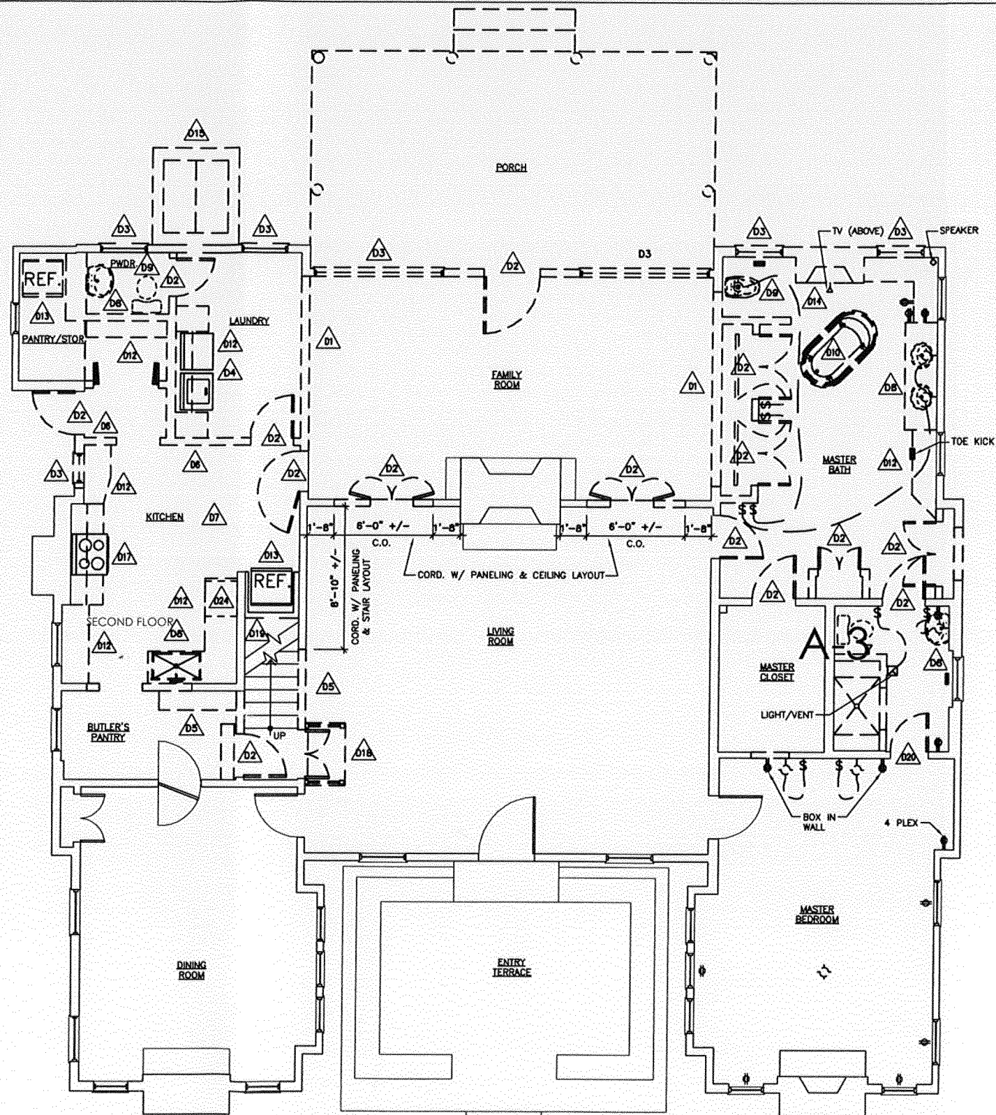
DEMOLITION PLAN 1/8" = 1'-0"
