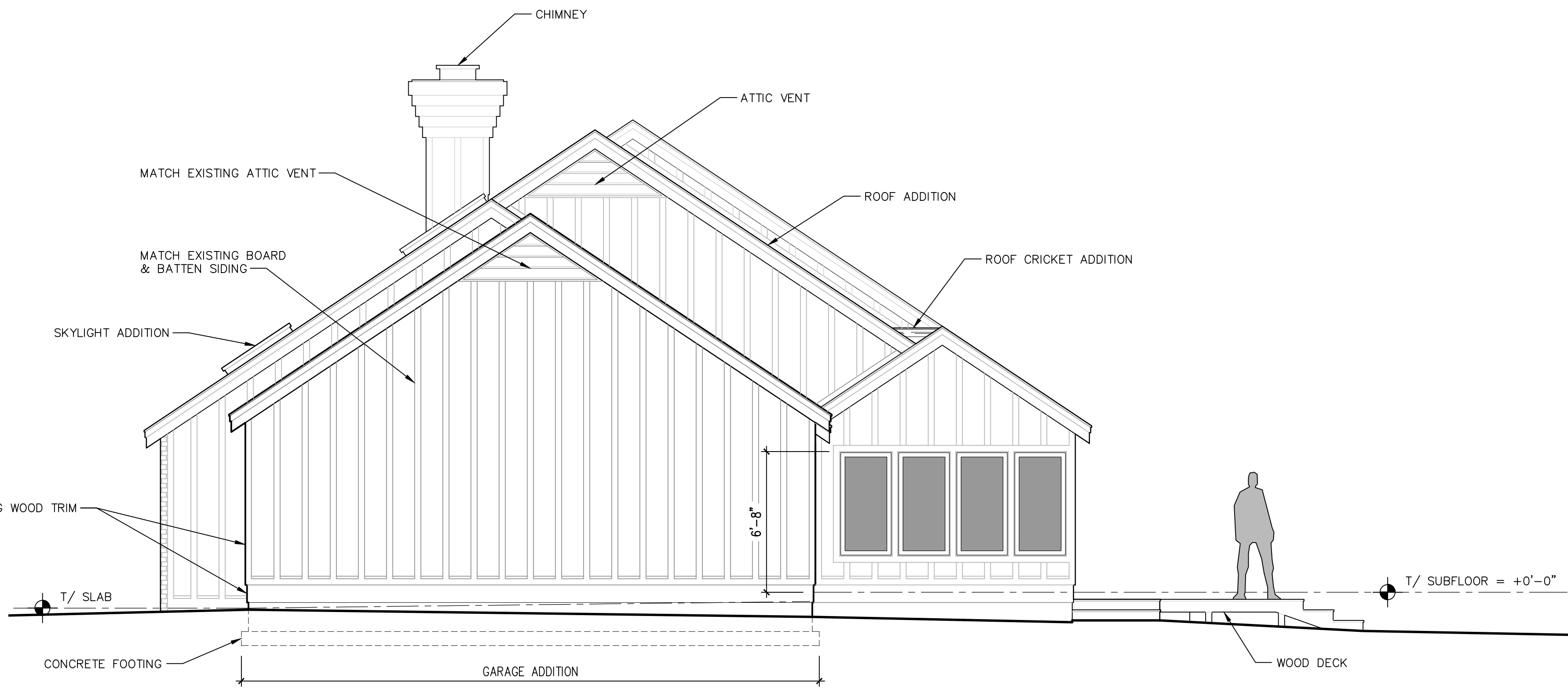
401 SOUTH ELEVATION
