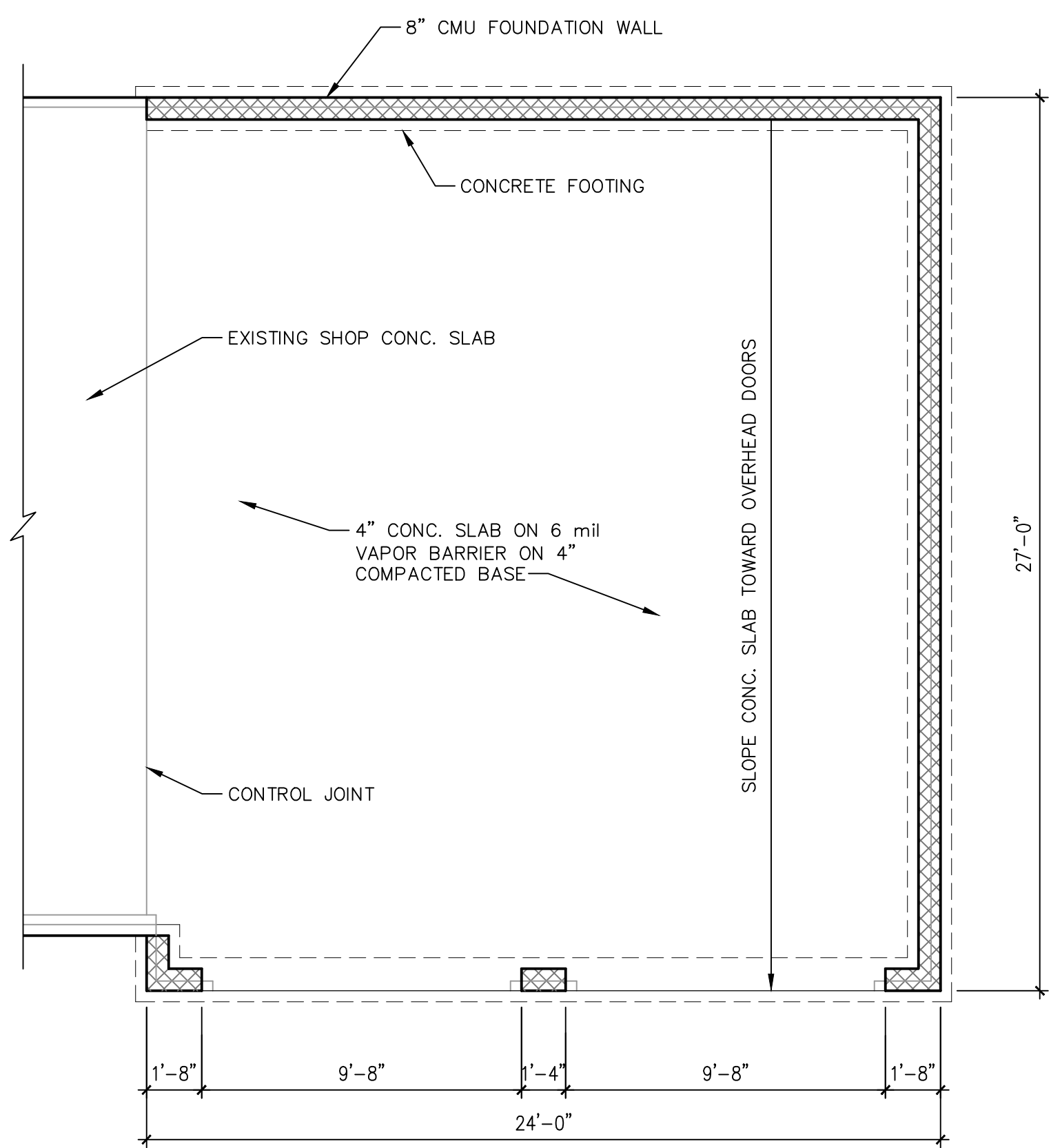
502 GARAGE ADDITION FOUNDATION PLAN
