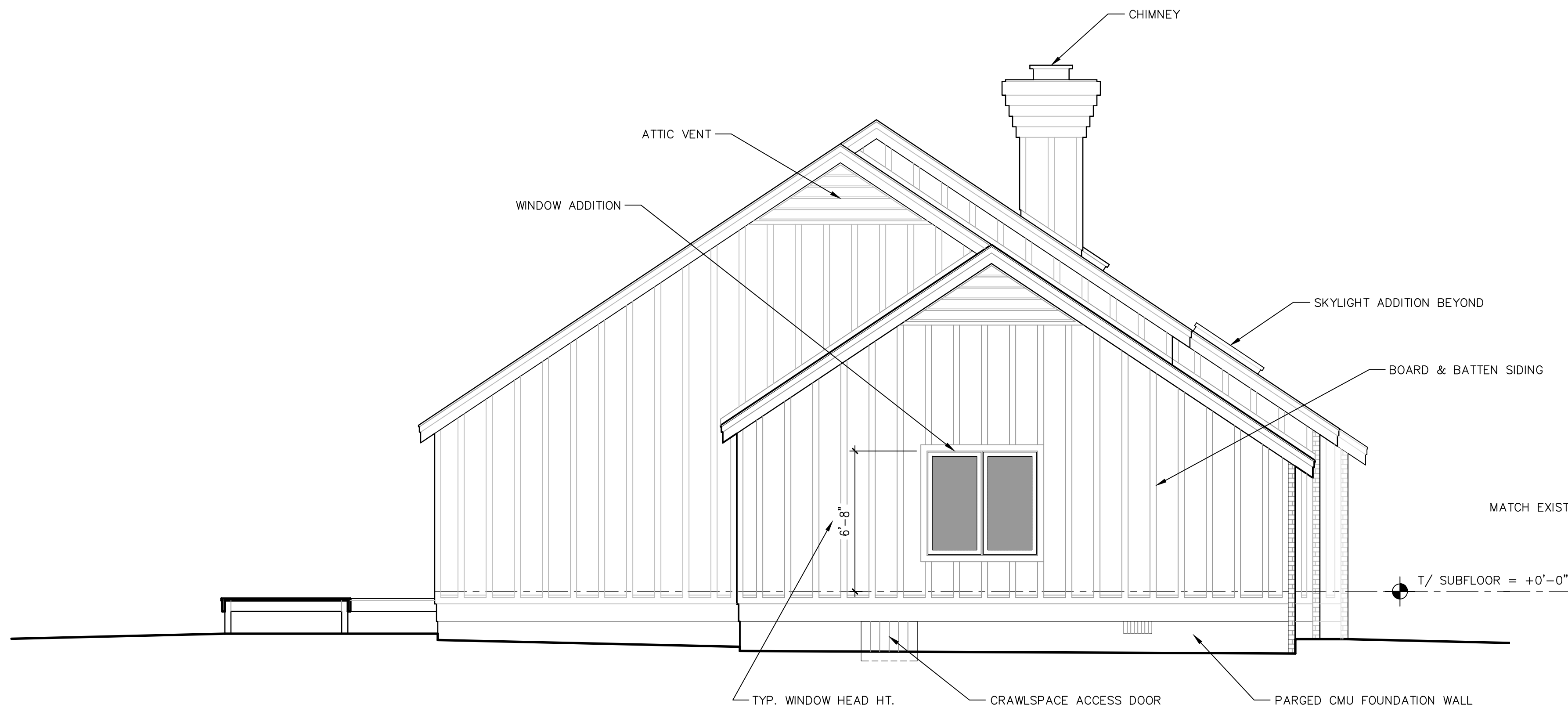
402 EAST ELEVATION
