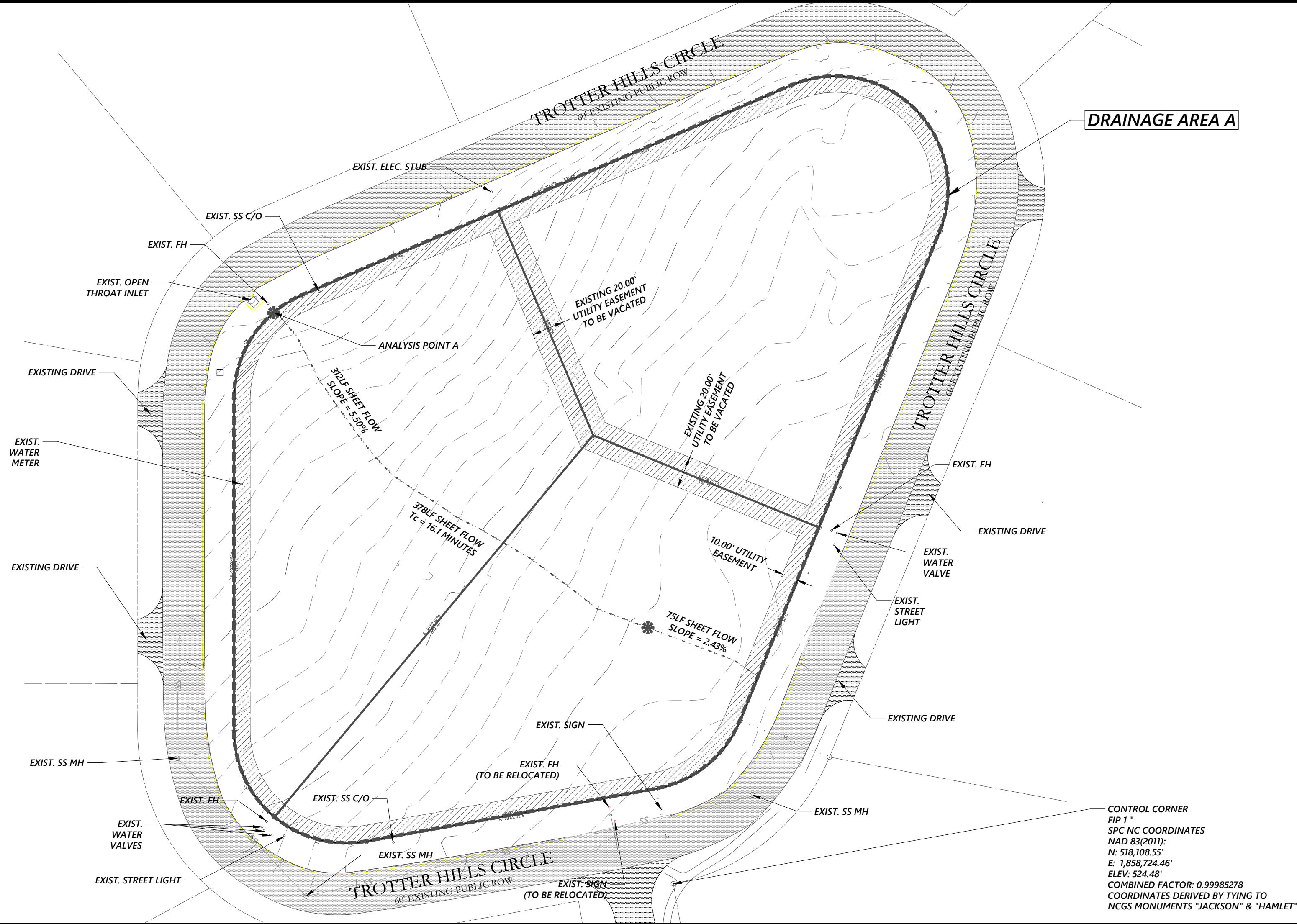
PRE DEVELOPMENT DRAINAGE AREA
