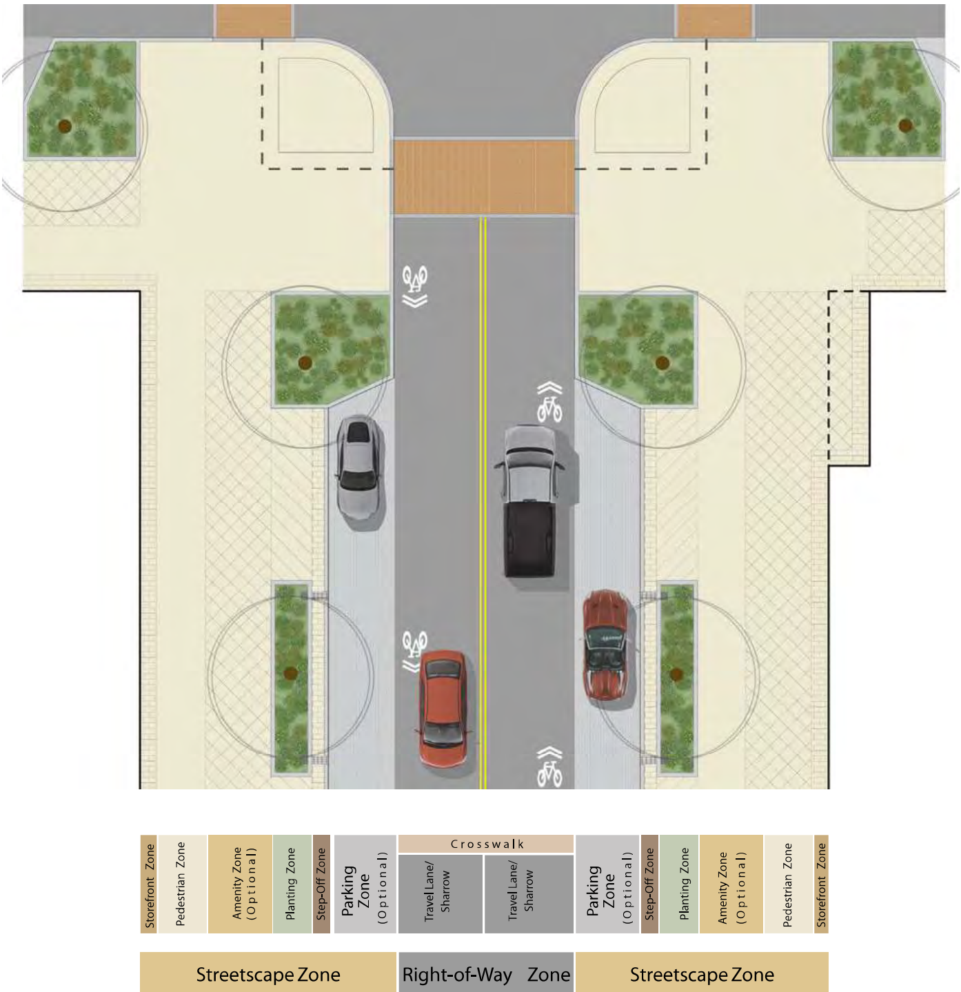
Complete Streets Diagram
