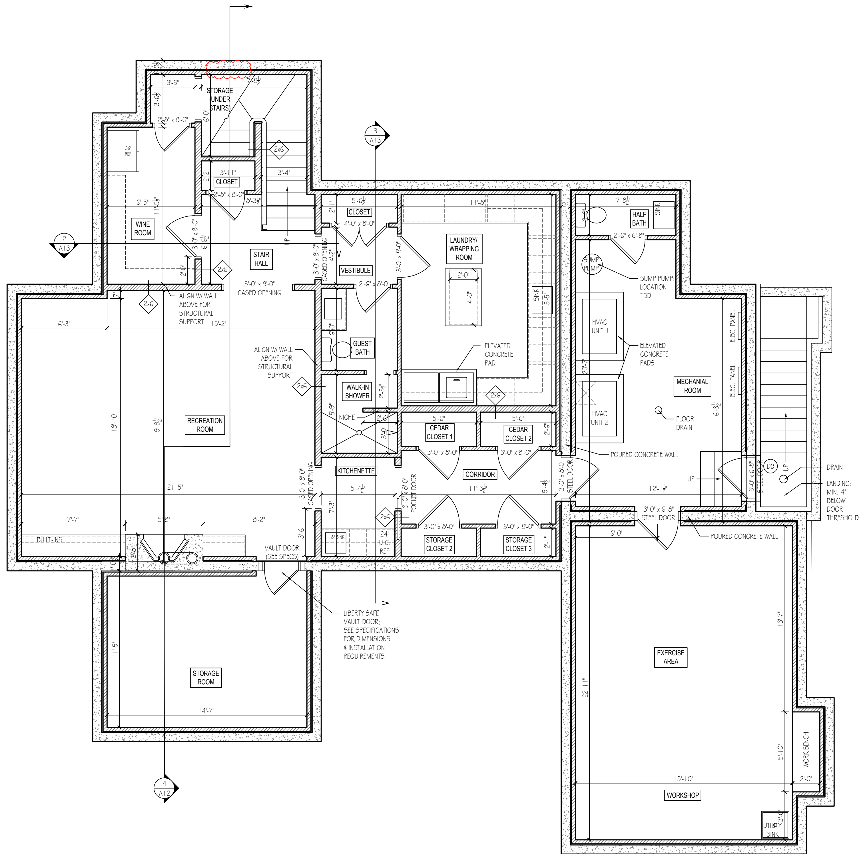
1 BASEMENT PLAN A7 SCALE: 1/4" = 1'-0"
