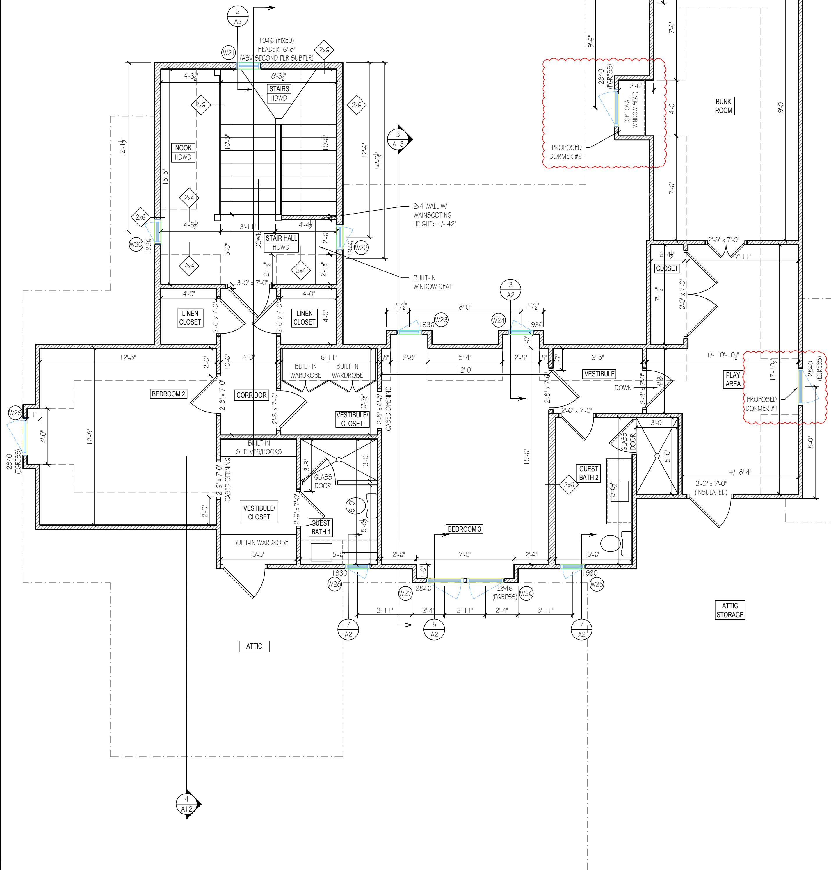
2 SECOND FLOOR PLAN A7 SCALE: 1/4" = 1'-0"
