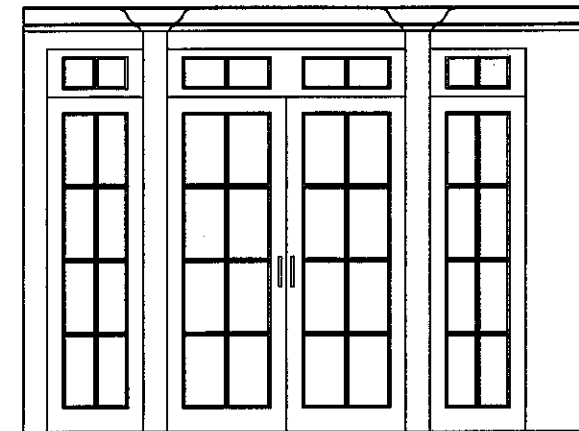
2 DINING ROOM WALL ELEVATION SCALE: 1/2" = 1'-0"
