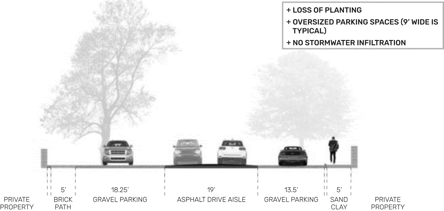
MAGNOLIA ROAD TYPICAL SECTION (WITHOUT VEGETATION)
