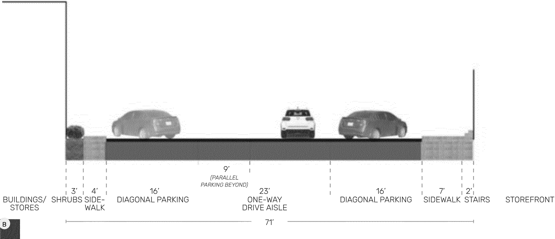
MARKET SQUARE TYPICAL SECTION (B)
