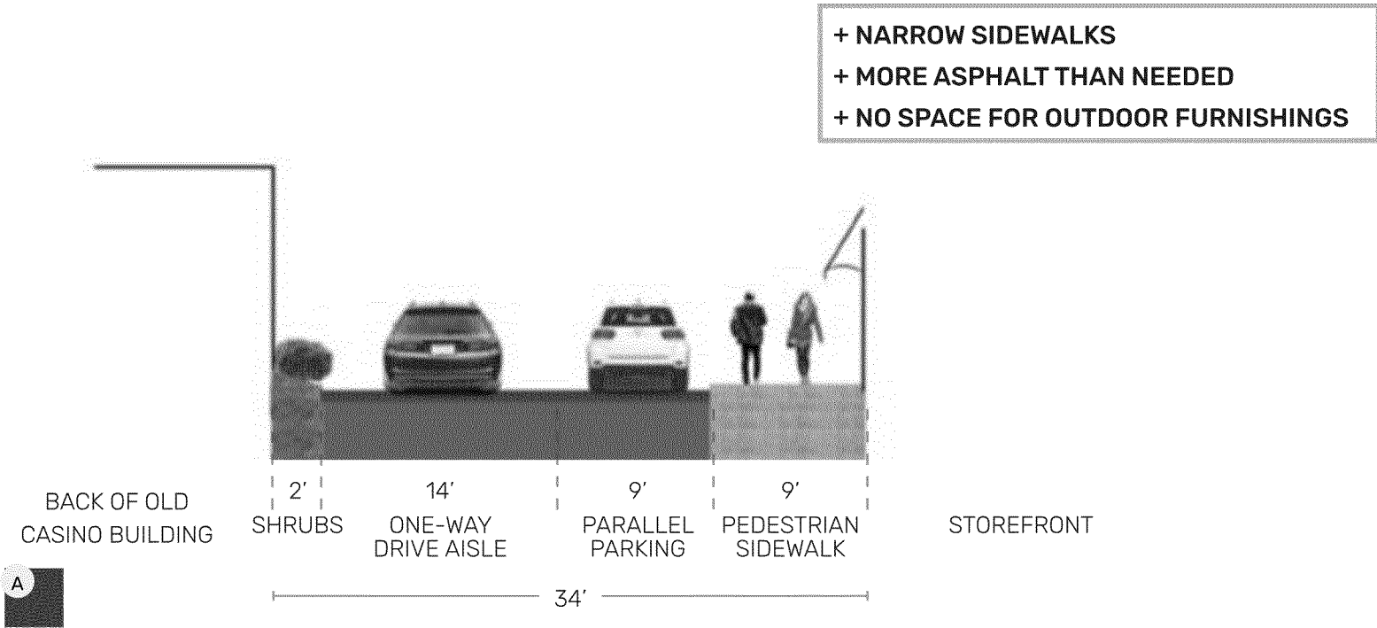
MARKET SQUARE TYPICAL SECTION (A)
