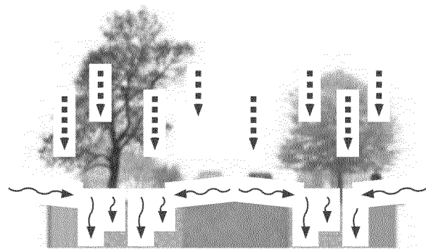
PROPOSED DRAINAGE PATTERN AT PARALLEL PARKING
