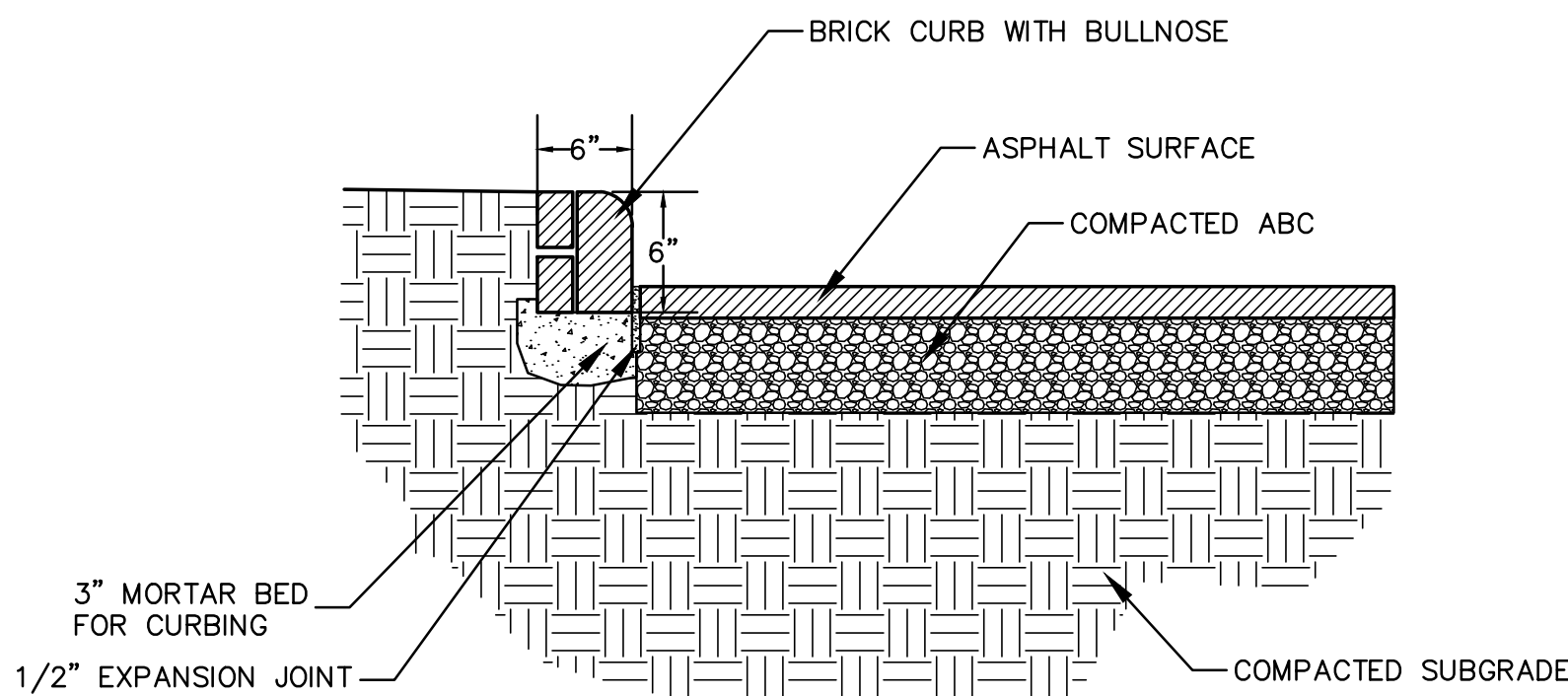
SECTION VIEW
