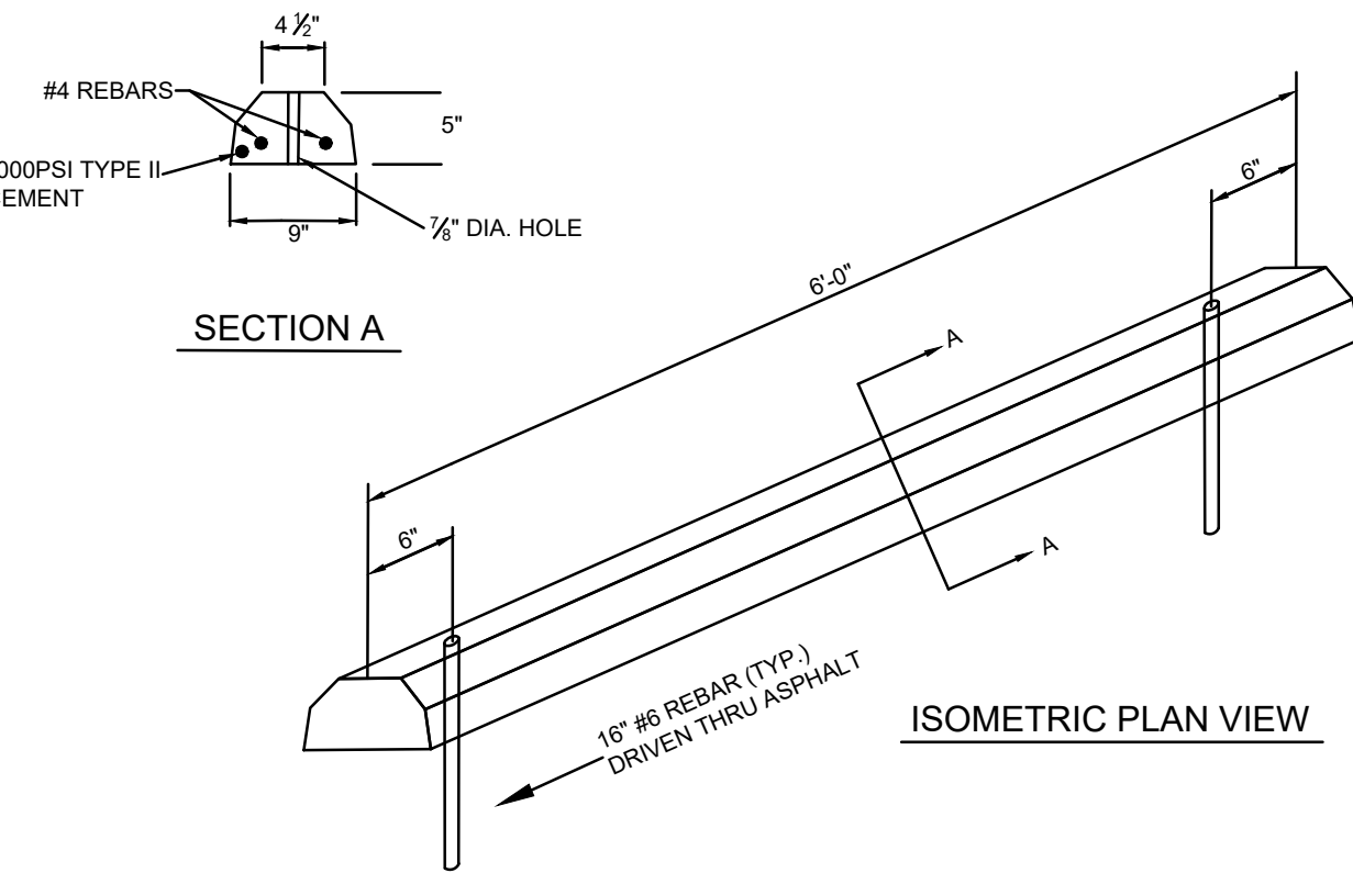
WHEEL STOP NOT TO SCALE
