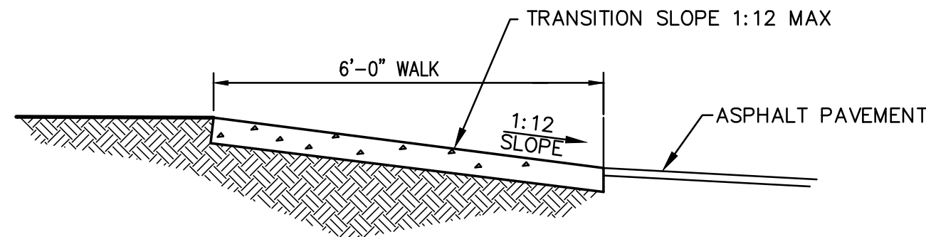
HANDICAP RAMP SECTION C
