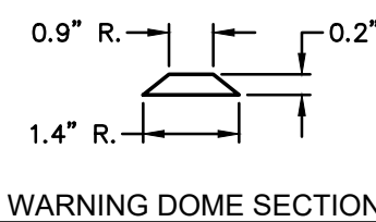
WARNING DOME SECTION
