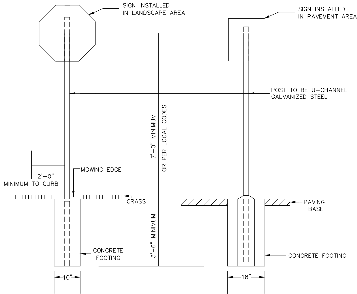
3 SIGN INSTALLATION
