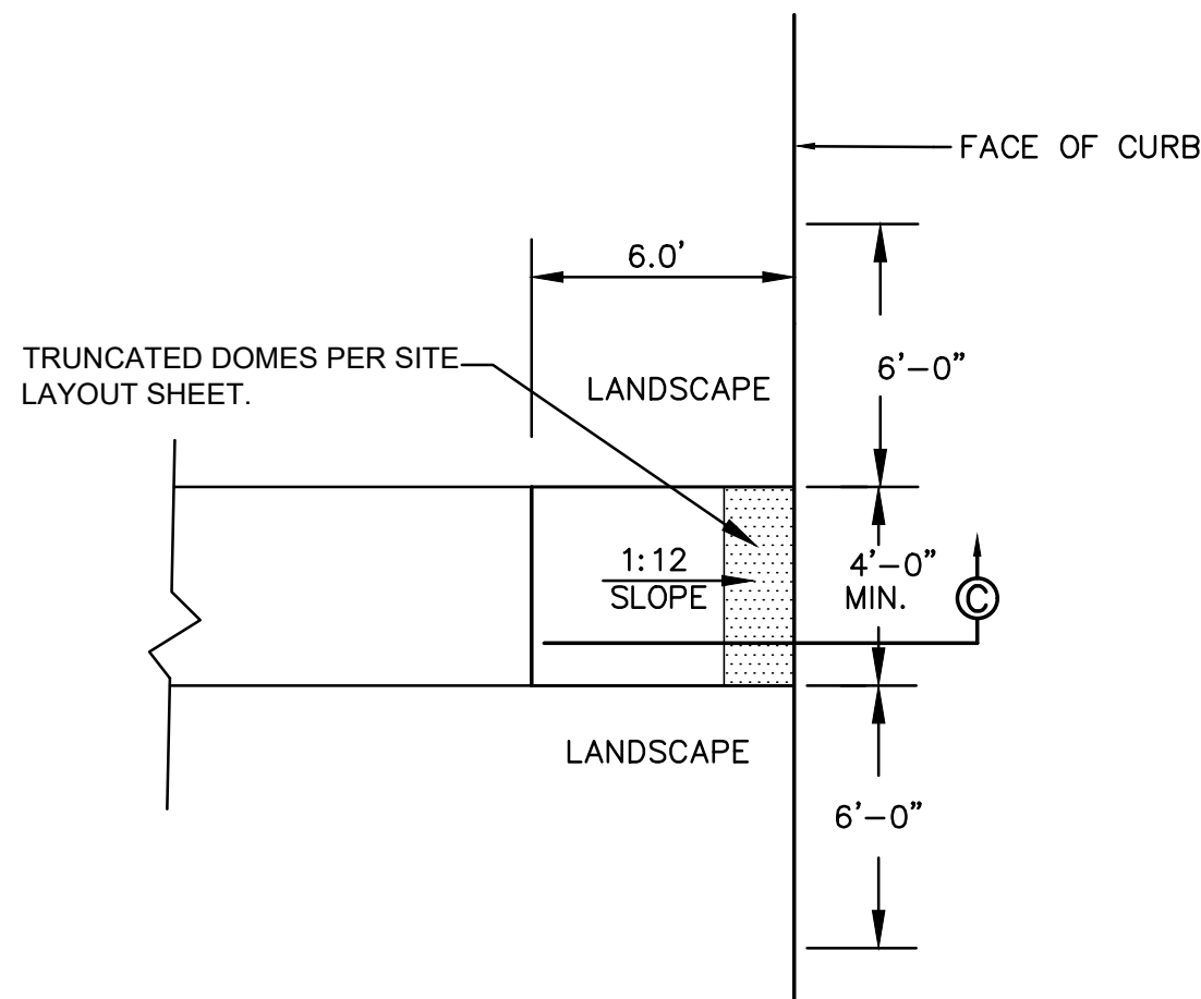
5 ACCESSIBLE RAMPS REVISED FOR THIS PROJECT NOT TO SCALE
