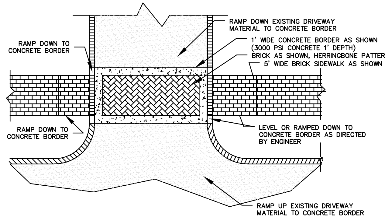
6 BRICK DRIVE APRON
