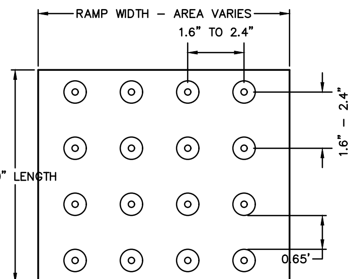
WARNING DOME SPACING
