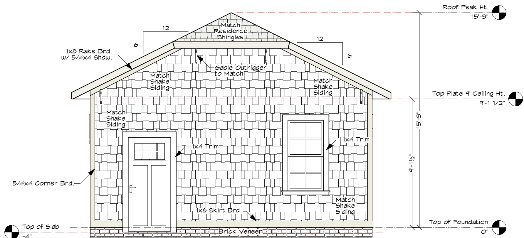
LEFT ELEVATION
