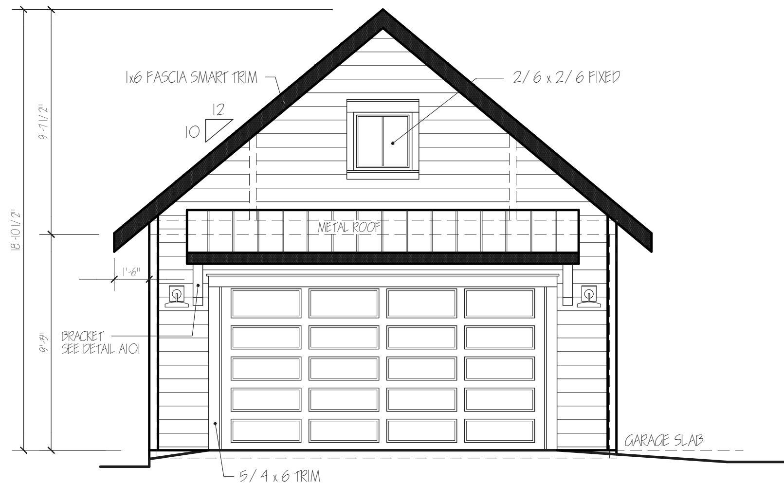
FRONT ELEVATION
