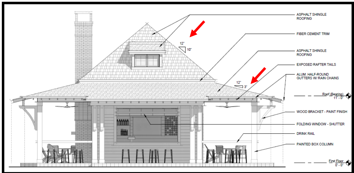
Front Elevation of the Pavilion
