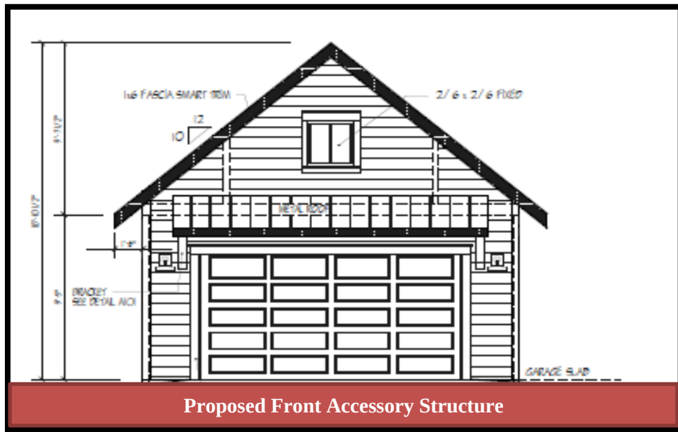
Front Elevation of 245 Magnolia
