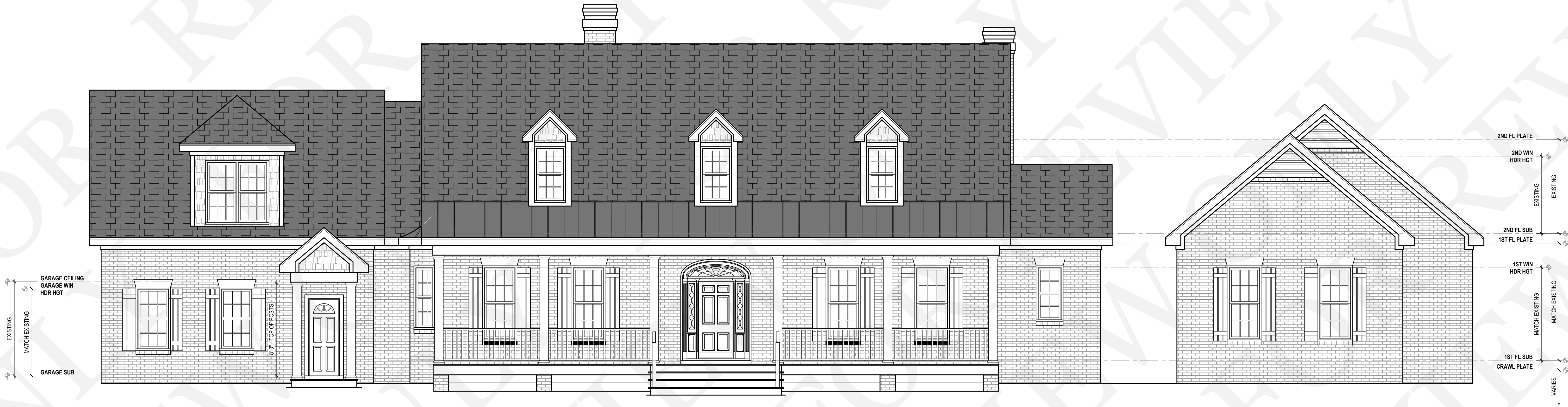
FRONT ELEVATION 1/4" = 1'-0"
