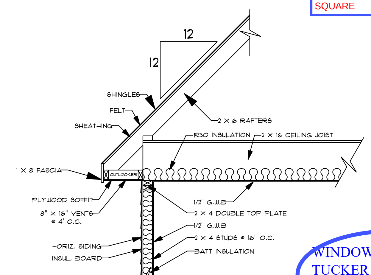
ROOF OVERHANG DETAIL SCALE: 1/2" = 1'
