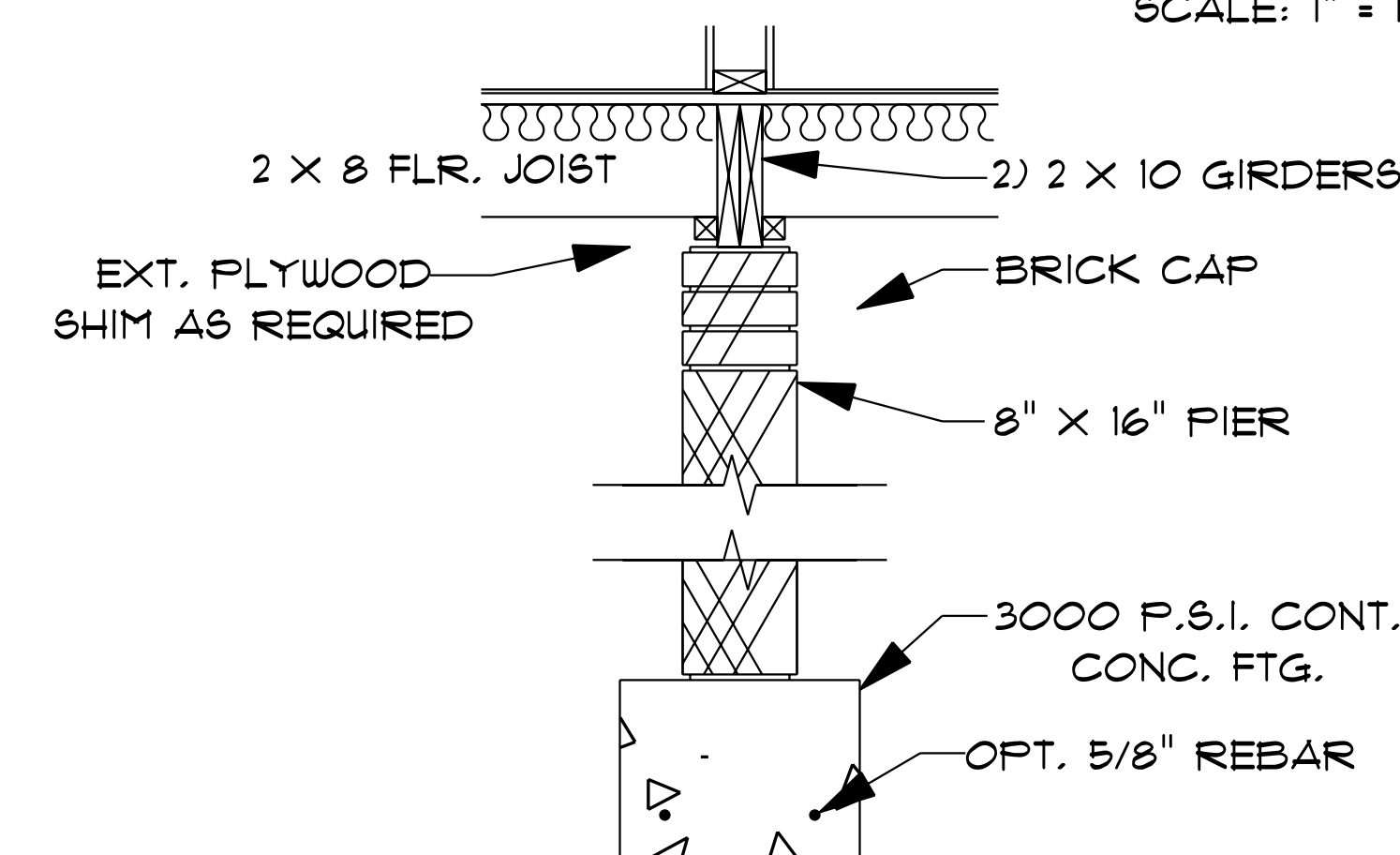
TYP. BEARING GIRDER SCALE: 1" = 1'0"
